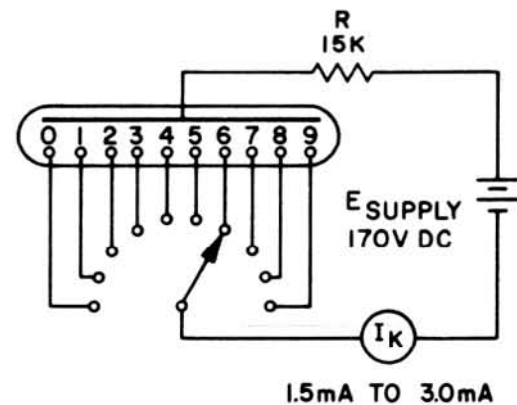
BASIC CIRCUIT
