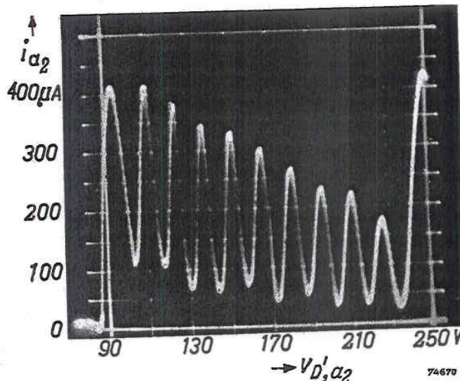
Fig. 10. Oscillographically 3) plotted i_{a_2} = f(v_{D,a_2}) characteristic of the EIT counter tube. Cf. curve 1 shown in fig. 6. The oscillogram displays one peak more than the theoretical curve shown in fig. 6. This is due to the fact that in practice a peak — the one the extreme left — also occurs when the beam passes between the slotted electrode and the reset anode. This peak is of no consequence for the operation of the tube.
