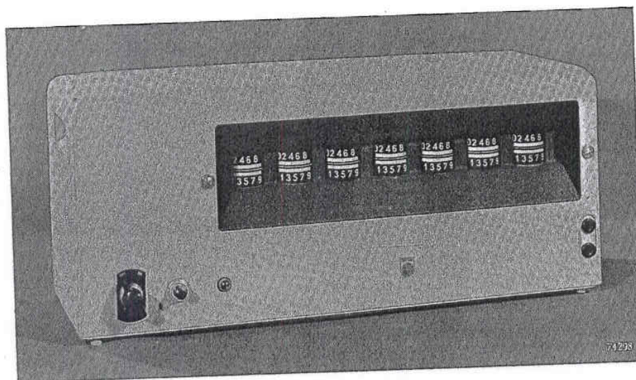
Fig. 2. Decade counter with seven decade counter tubes EIT connected in cascade, suitable for counting up to (10^7 - 1) at a speed of 30,000 pulses per second. From left to right the millions, the hundred thousands, the ten thousands, etc. can be read on the tubes themselves. Bottom left: mains switch, push-button switch with which all counter tubes can be reset to zero before counting starts, and pilot lamp. Bottom right: input terminals.
