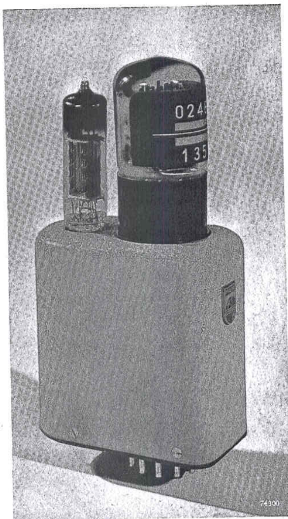
Fig. 18. A decade counter tube with its accessory pulse shaper connected according to the circuit of fig. 16, in the form of a unit 6) to be inserted in a tube holder.
