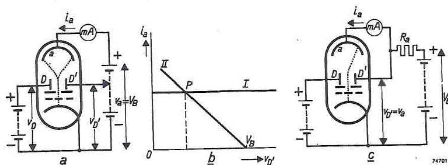
Fig. 4. (a) Imaginary cathode-ray tube with an electron gun, deflection electrodes D , D' and an anode a . At v_a and v_D = \text{constant} , the electron beam can be given any position between the extreme positions (dotted lines) by varying v_{D'} . In doing so the anode current i_a remains constant, see I in (b).
