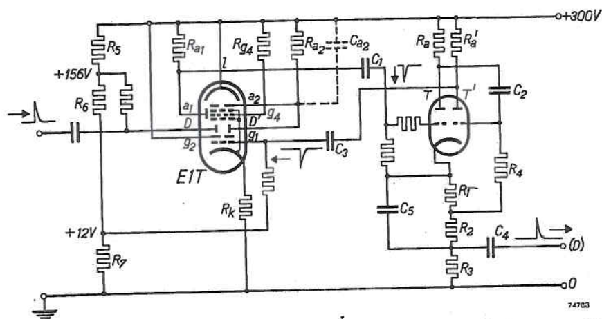
Fig. 16. Circuit of a counter tube and the following pulse shaper. The latter is a monostable (one-shot) multivibrator (flip-flop) incorporating a double triode T - T' (type E 90 CC).
