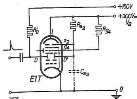
Fig. 5. EIT counter tube of which the anode a_2 and the deflection electrode D' are fed via a common resistor R_{a_2} , similar to the tube shown in fig. 4c. The beam has now the same number of stable positions as the number of slots in the electrode g_4 (see also fig. 6). By applying positive pulses to D , the beam can be advanced in steps (see later). C_{a_2} represents the stray capacitance.
