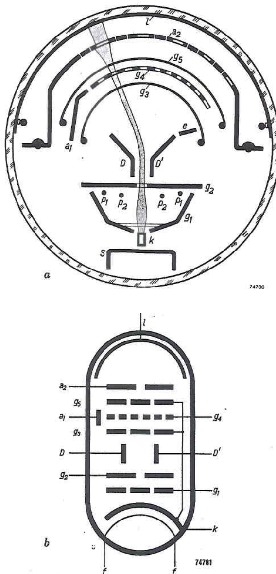
Fig. 3. (a) Cross section and (b) diagrammatic representation of the decade counter tube. The cathode k (with heater f ), the control grid g_1 , the four internally connected focusing electrodes p_1 and p_2 and the accelerating electrode g_2 form the electron gun, which produces a ribbon-shaped electron beam (the width of the ribbon is normal to the plane of the drawing). D, D' deflection electrodes, g_3, g_5 suppressor grids, a_1 reset anode, g_4 electrode with ten slots, a_2 anode, l fluorescent layer applied to a conductive layer. Screen s (internally connected to k ) prevents primary electrons from impinging on the envelope. Auxiliary anode e (internally connected to g_2 ) captures secondary electrons.
