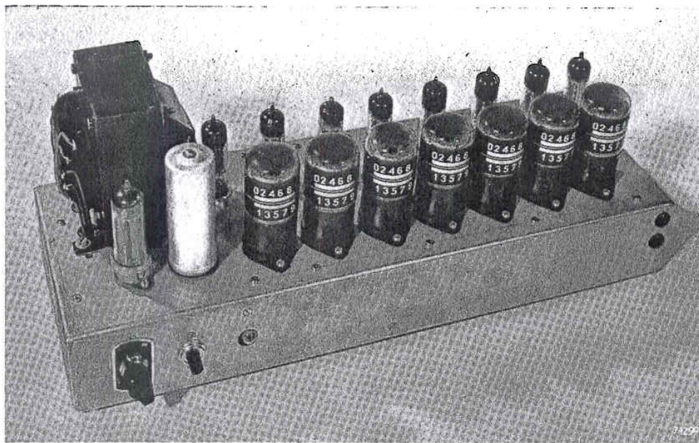
Fig. 15. The decade counter depicted in fig. 2 with the cover removed. Behind the seven EIT counter tubes the eight double triodes E90CC, which act as pulse shapers, can be seen. At the left is the rectifier valve AZ 41 which provides the direct current for the entire apparatus (300 V, approximately 50 mA).
