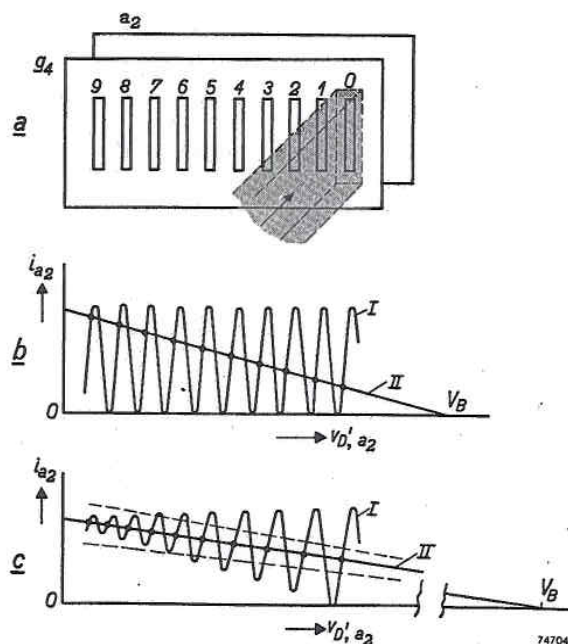
Fig. 7. (a) a_2 anode and g_4 slotted electrode of a (primitive) decade counter tube, both drawn as flat planes. The ten slots have been drawn as being of the same size and equidistant. (b) Curve I: i_{a2} = f(v_{D', a_2}) characteristic which might be expected in the case (a). II again represents the resistance line. (c) Due to the defocusing of the beam as it is deflected to the left, the i_{a2} = f(v_{D', a_2}) characteristic actually assumes the form represented by I. At small variations of R_{a2} (corresponding to the broken lines) some of the points of intersection at the left are lost. V_B must, moreover, largely exceed the value of v_{D', a_2} corresponding to the point of intersection 0.
