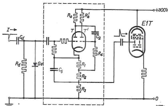
Fig. 20. Circuit of the input pulse shaper. I applied negative-going counting pulses. C_d - R_d differentiating network. Ge germanium diode (type OA 55), which prevents a positive voltage occurring across R_d . The circuit within the rectangle corresponds to that shown in fig. 16 of the other pulse shapers. At the right of this circuit is the first counter tube.
